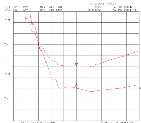
SWR(S11 & S22)
