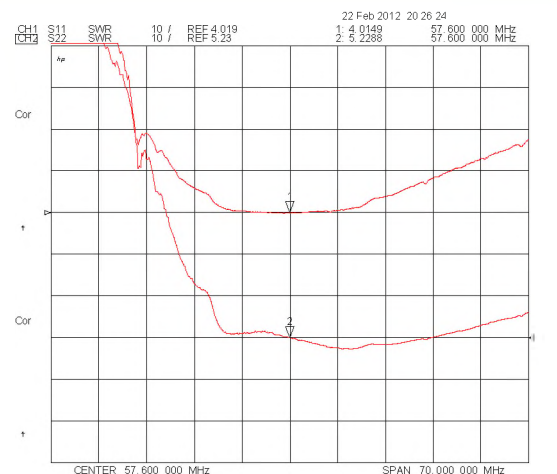
SWR(S11 & S22)
