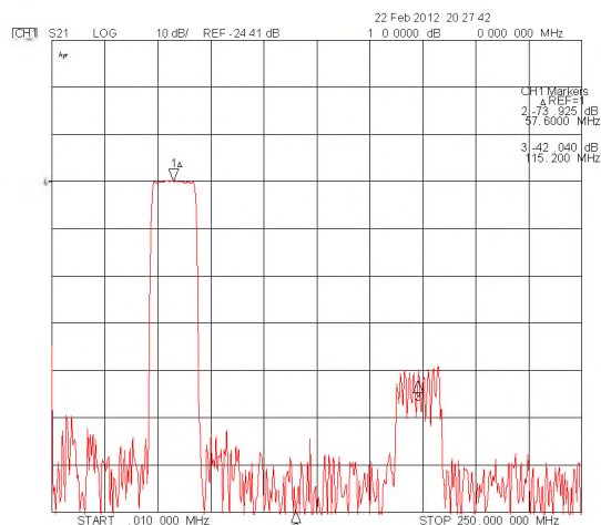
Wideband Properties
