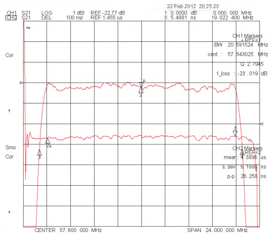
Wideband Properties
