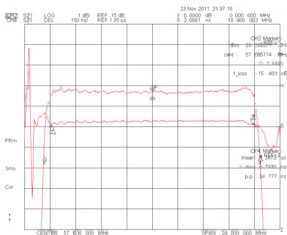
Relative Attenuation(Fo – 13.8 MHz)
