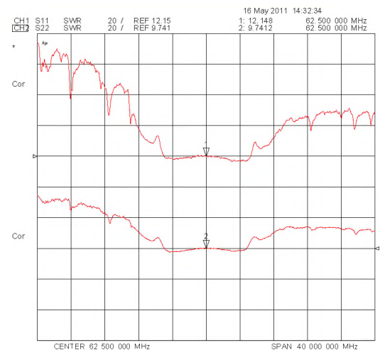
SWR(S11 & S22)
