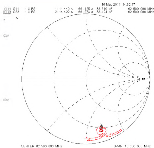
Smith Chart
