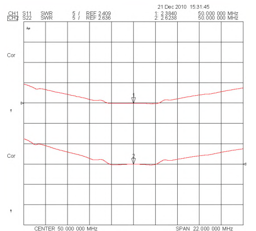
SWR(S11 & S22)
